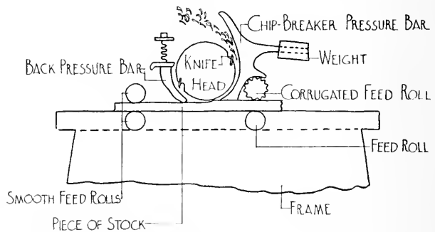
FIG. 155. SECTION THRU A SURFACER.
